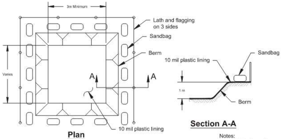
Type "Below Grade"
